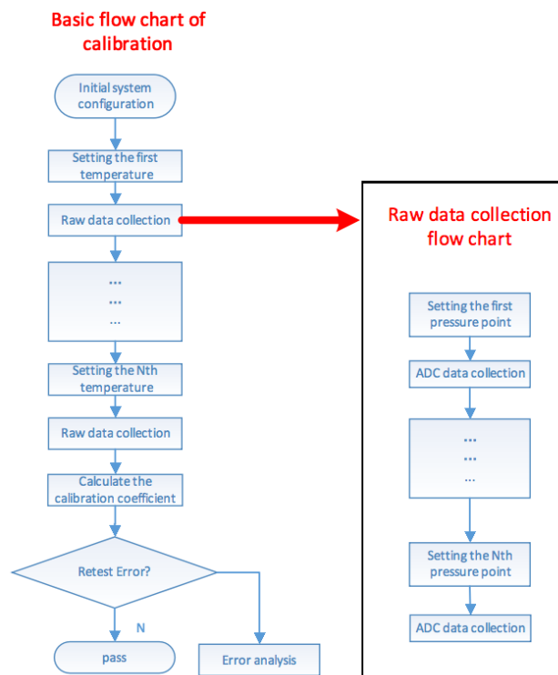
Figure 7.1 Sensor calibration process
