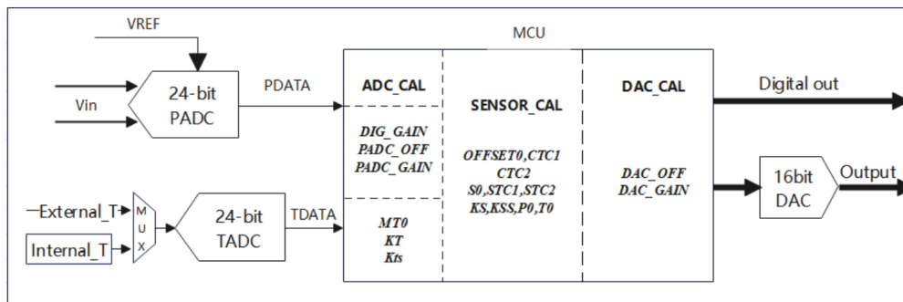
Figure1.1 NSA(C)9260X SIGNAL CHAIN
